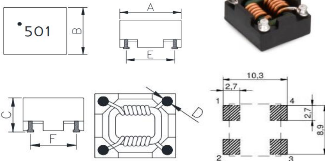
Land Pattern
