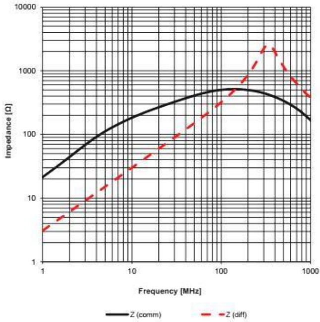
BCCM1005-2-501T
