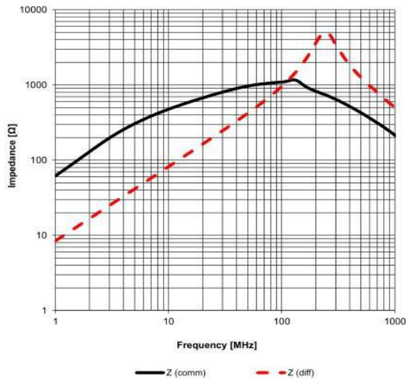
BCCM1005-2-102T
