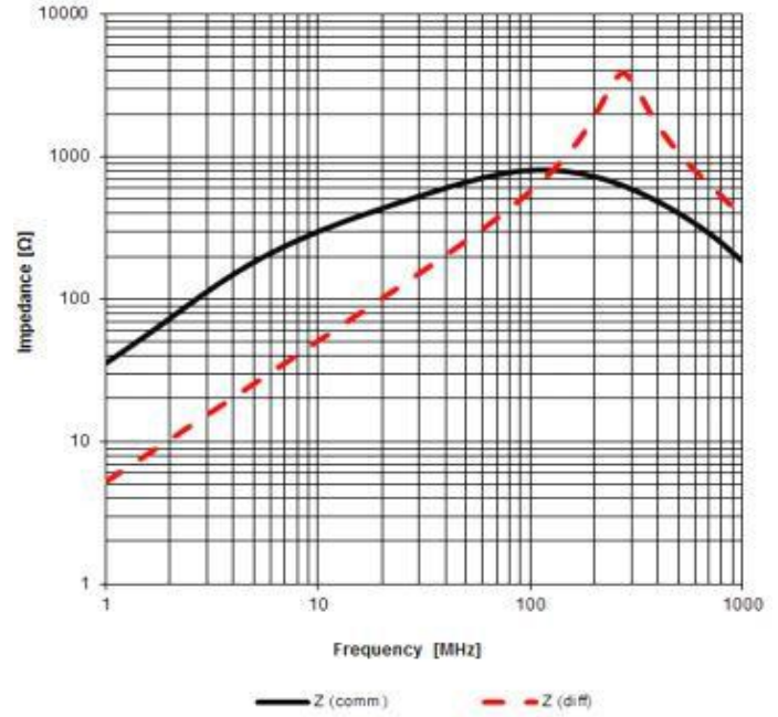
BCCM1005-2-801T
