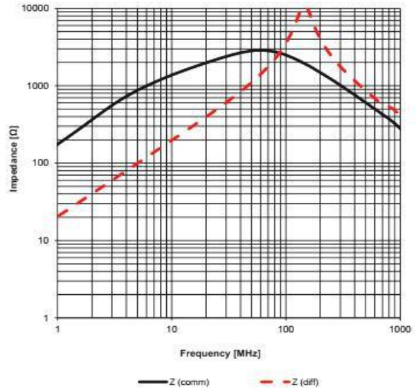
BCCM1005-2-222T
